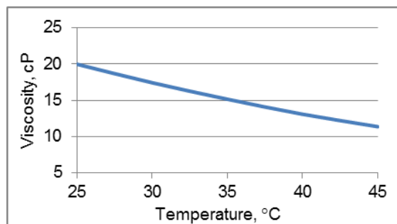
Viscosity Profile
