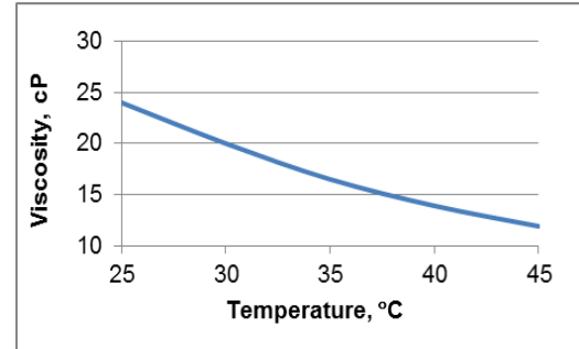
Viscosity profile
